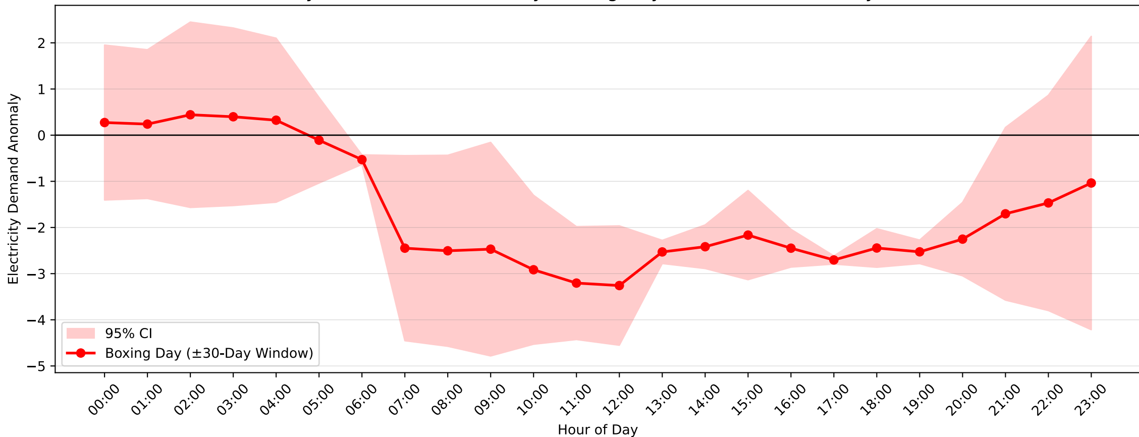
Dee Why West Demand Anomaly: Boxing Day (2014-2015, \pm 30 -Day Window)
